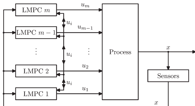
Figure 3. Iterative distributed LMPC.
